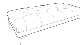
Deep Buttoned Stool Width: 128cm Depth: 64cm Height: 33cm
